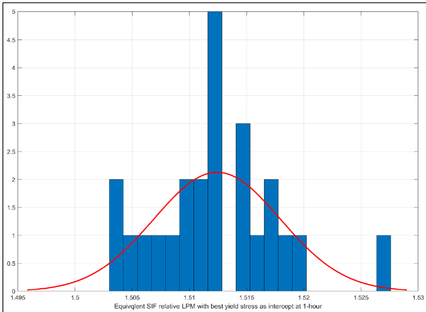
Figure 19: PE2708 LTHS SIF histogram with normal distribution fit. Mean SIF=1.5124.
