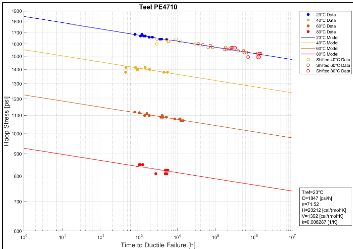
Figure 16: PE4710 LTHS test results. LPM parameters are shown in bottom right text box.
