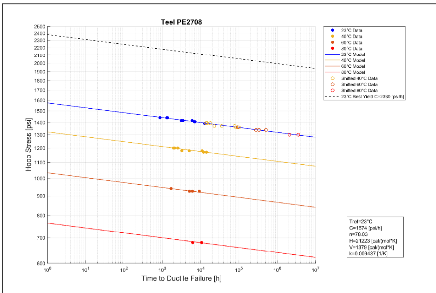
Figure 17: PE2708 LTHS test results with "best yield reference curve.
