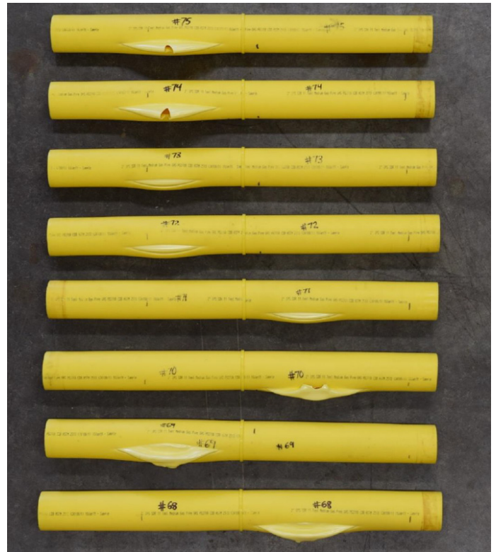
Figure 11: Teel's 2710 and 2708 quick burst test samples after testing
