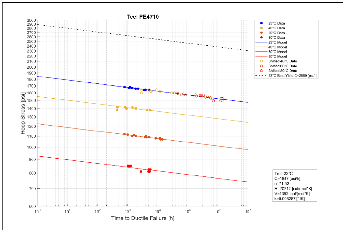
Figure 18: PE4710 LTHS test results with "best yield reference curve.
