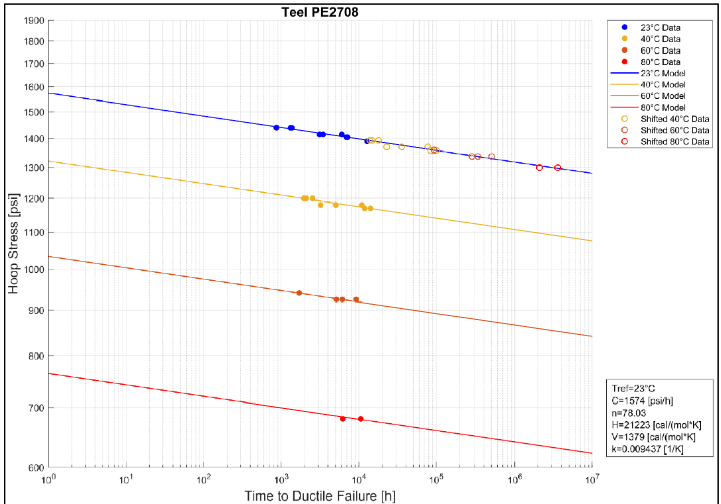
Figure 15: PE2708 LTHS test results. LPM parameters are shown in bottom right text box.
