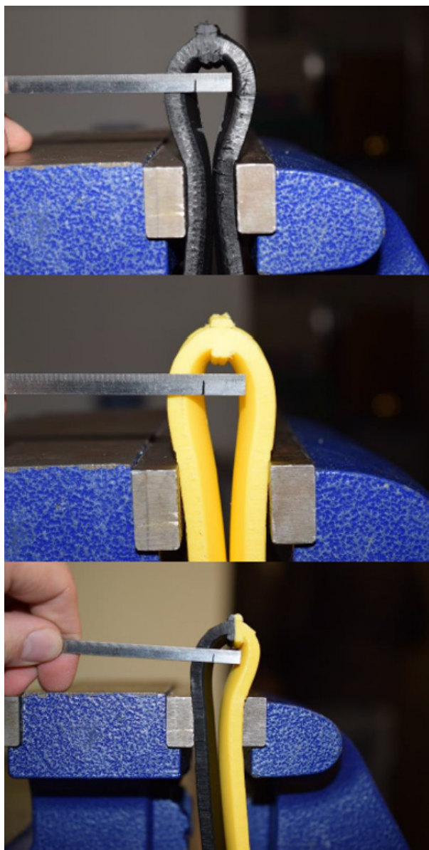
Figure 10: Teel's bend back test samples after testing
