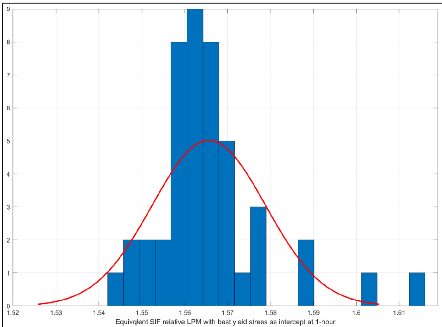
Figure 20: PE4710 LTHS SIF histogram with normal distribution fit. Mean SIF=1.5656.
