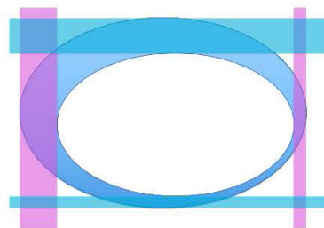
12-If the ellipse is not perfectly round, we see a more realistic example as above: A. Position of both ellipses are clearly defined. B. Eccentricity and ovality can clearly be identified C. This allows determination of the wall-thickness at every point.
