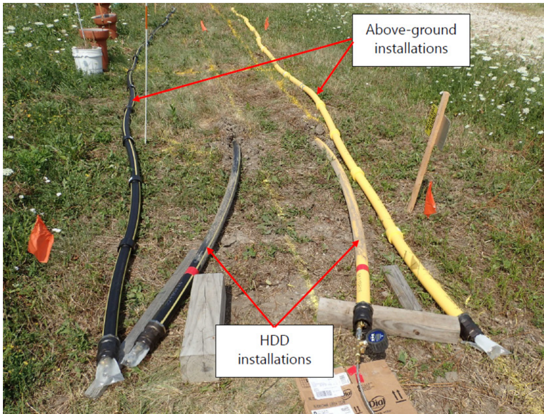
Figure 13: Completed above-ground and HDD installations
